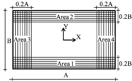
Figure 3. Plan of a typical building showing requirement of minimum 20% of the total length of lateral load-resisting walls along both x and y directions to be placed in each of the external frames in both directions (NBC-201 1995).
